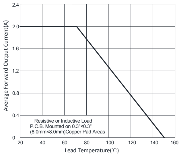
FIG1: Io-TL Curve
